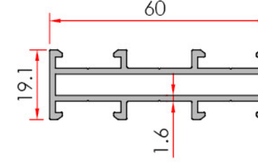
Narrow Frame Dar Kasa
