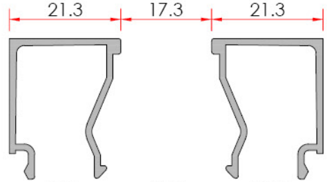
Bead - Çıta System Code 22 G 03 Profile No 1368 Weight kg/m 0.285
