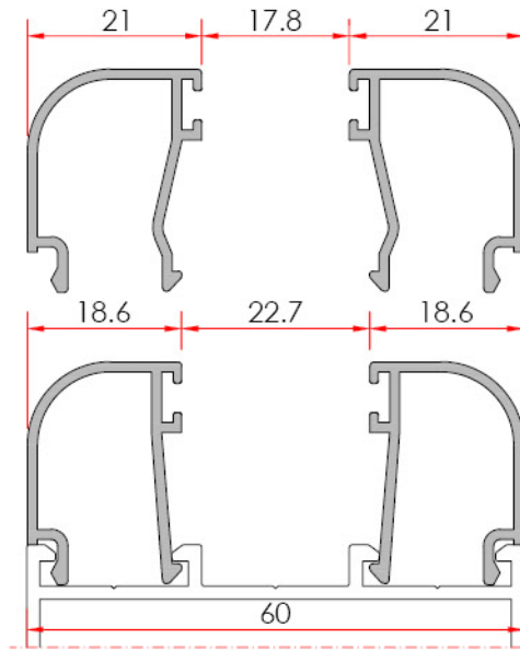
Bead - Çıta System Code 22 RG 02 Profile No 1957 Weight kg/m 0.264
