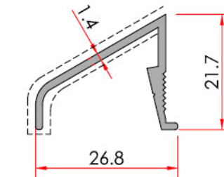
Drainage Damlalık
