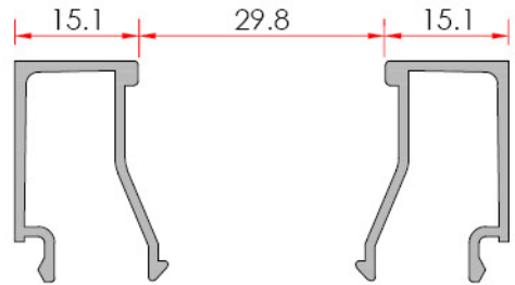
Bead - Çıta System Code 22 G 07 Profile No 1611 Weight kg/m 0.261
