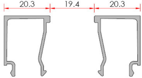
Bead - Çıta System Code 22 G 02 Profile No 1366 Weight kg/m 0.278
