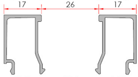
Bead - Çıta System Code 22 G 09 Profile No 1613 Weight kg/m 0.268
