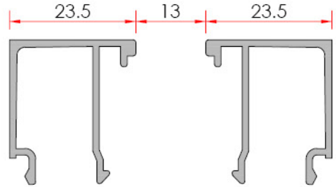
Bead - Çıta System Code 22 G 11 Profile No 1616 Weight kg/m 0.300
