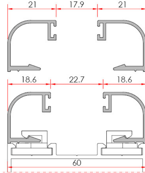
Bead - Çıta System Code 22 RK 02 Profile No 1959 Weight kg/m 0.228
