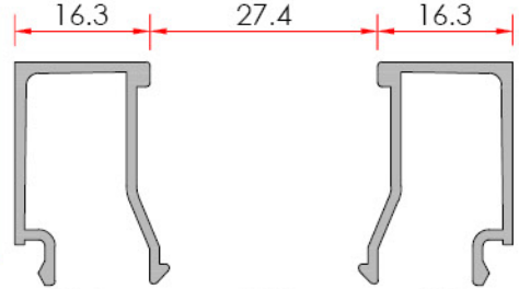
Bead - Çıta System Code 22 G 01 Profile No 1367 Weight kg/m 0.265
