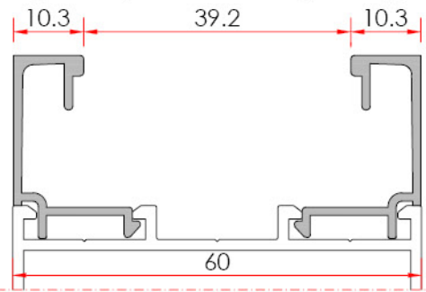
Bead - Çıta System Code 22 G 10 Profile No 1378 Weight kg/m 0.228
