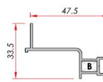
Spandrel Panel Spandrel Paneli
