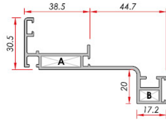
Hidden Wing Frame Gizli Kanat Kasa Panel
