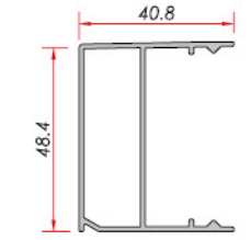
Cover Yatay Kapak
