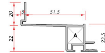
Composite Panel Kompoze Panel
