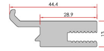
Glass Wedge Cam Takozu
