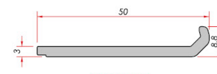
Glass Wedge Cam Takozu
