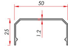
Cover Dikey Kapak
