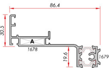
Hidden Wing Frame Gizli Kanat Kasa Panel
