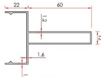
Cover Dikey Kapak
