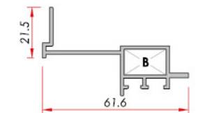
Composite Panel Kompoze Panel
