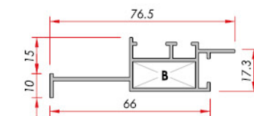
Composite Panel Kompoze Panel
