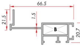
Spandrel Panel Spandrel Paneli
